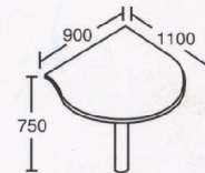
IR-CT1100 Connection Top with Metal Leg (Left & Right) L1100 x W900 x H750
