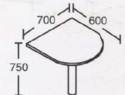
IR-HRCT70 Half Round Connection Top with Metal Leg L600 x W700 x H750
